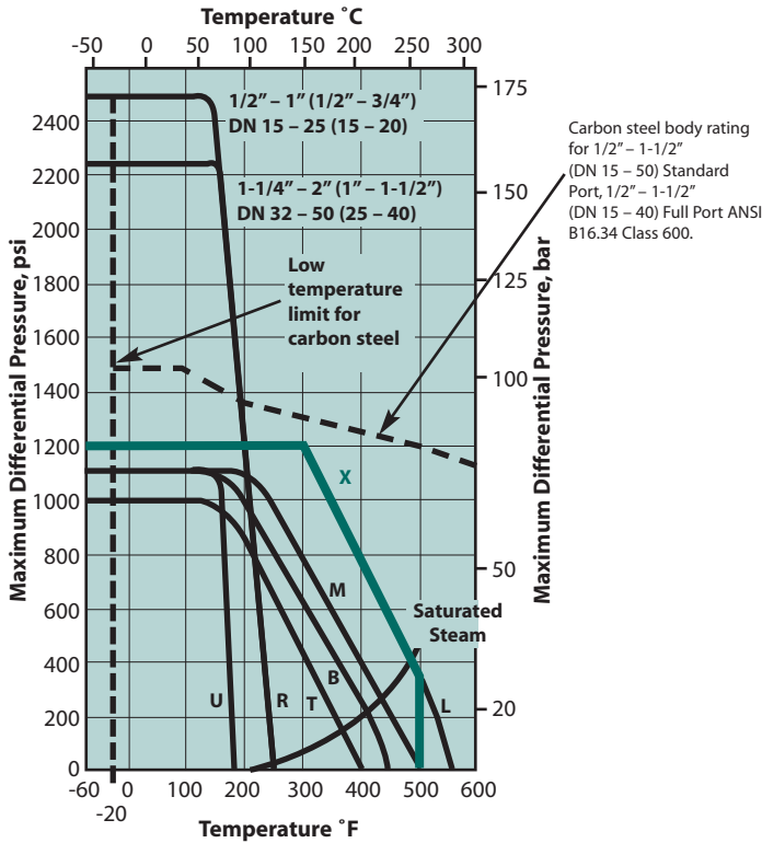
1/2" – 2" (DN 15-50) Standard Port, 1/2" – 1-1/2" (DN 15-40) Full Port Valves
