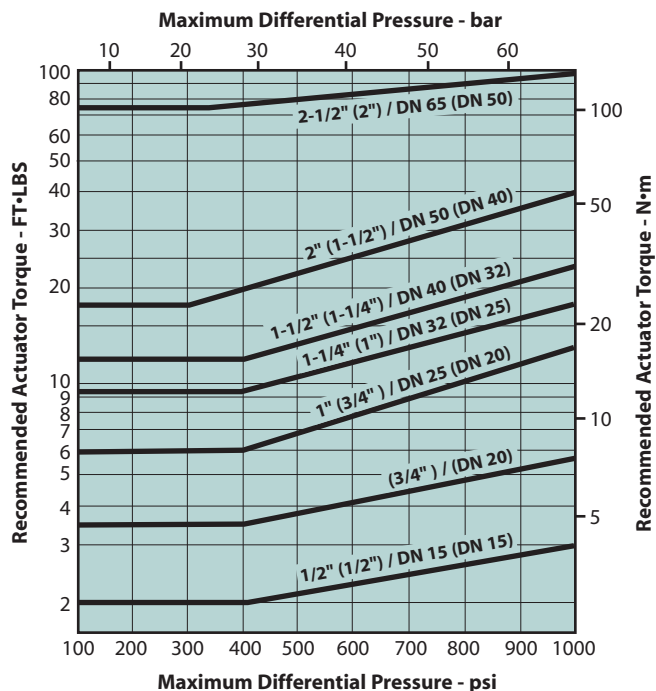
PTFE (T) Seated Standard-Port Valves
