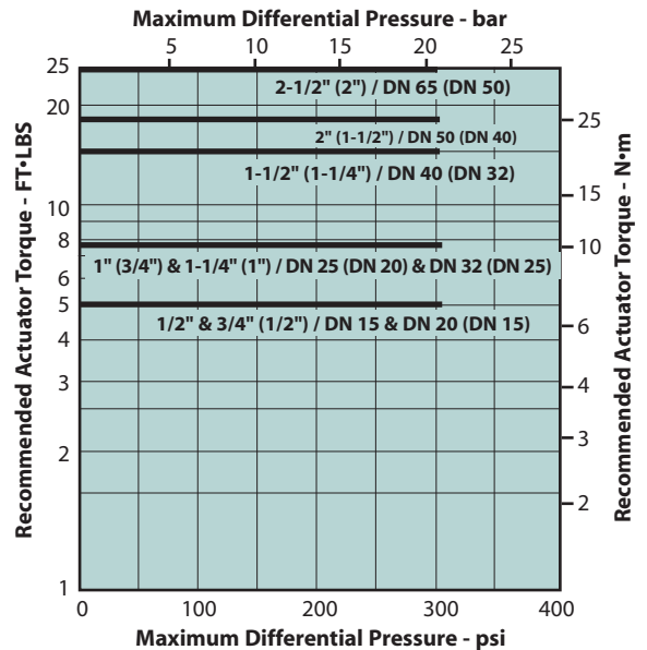
Metal (D) Seated Standard-Port Valves (Full-port sizes in parentheses)
