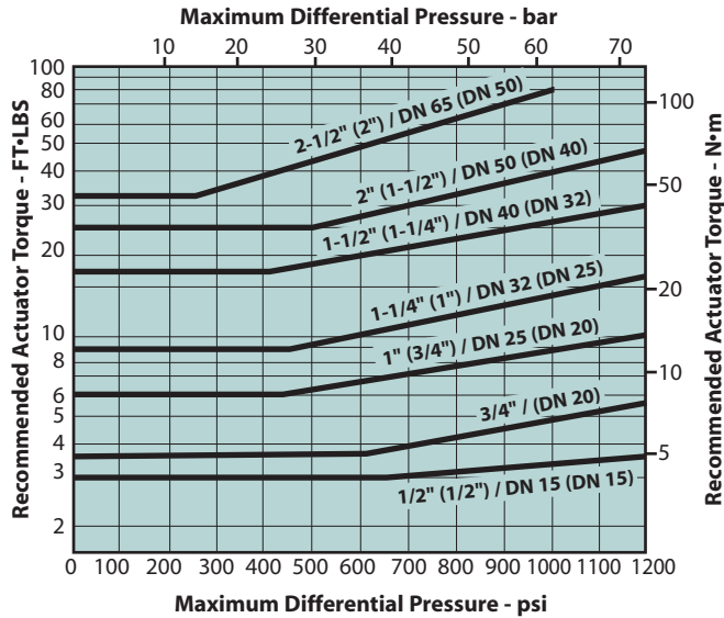
XTREME (X) Seated Standard-Port Valves (Full-port sizes in parentheses)
