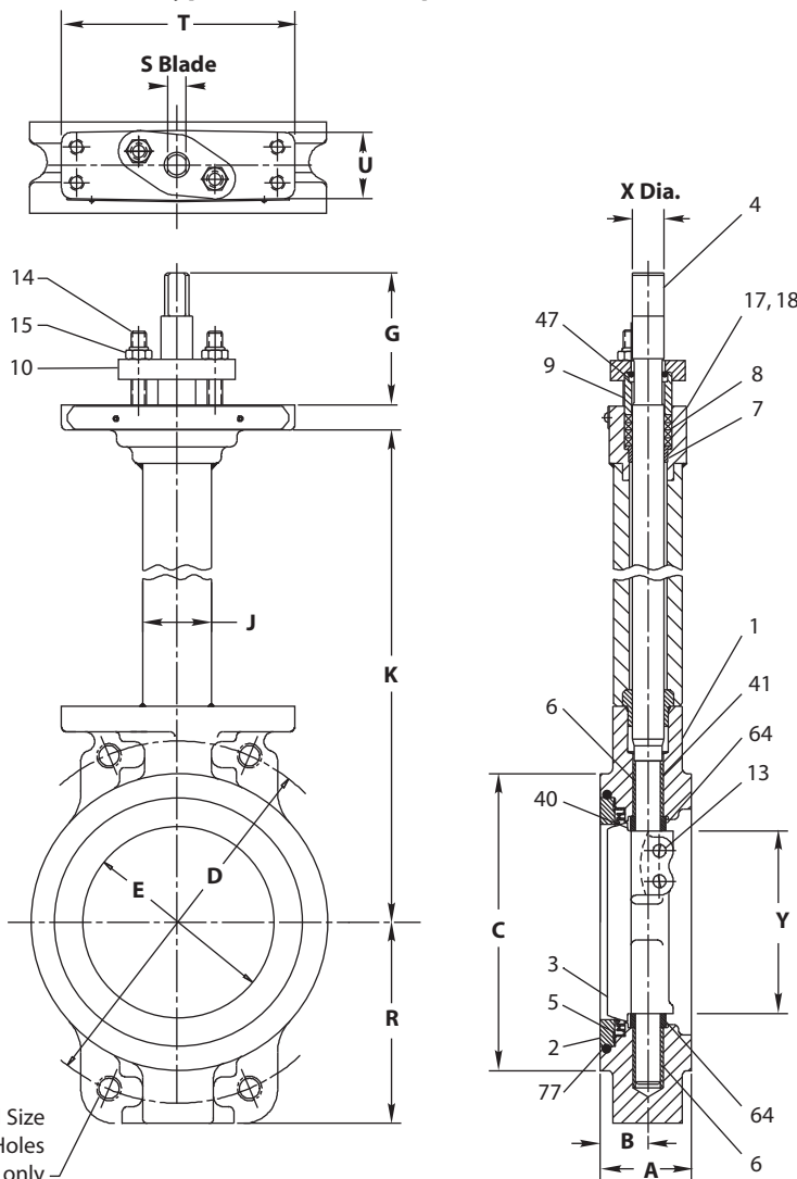
3" – 12" (DN 80 – 300) Type K830W Wafer-Sphere Valves ANSI Class 300 Wafer Design
