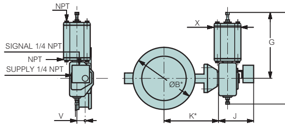
STANDARD MOUNTING POSITION
