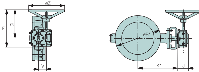
STANDARD MOUNTING POSITION
